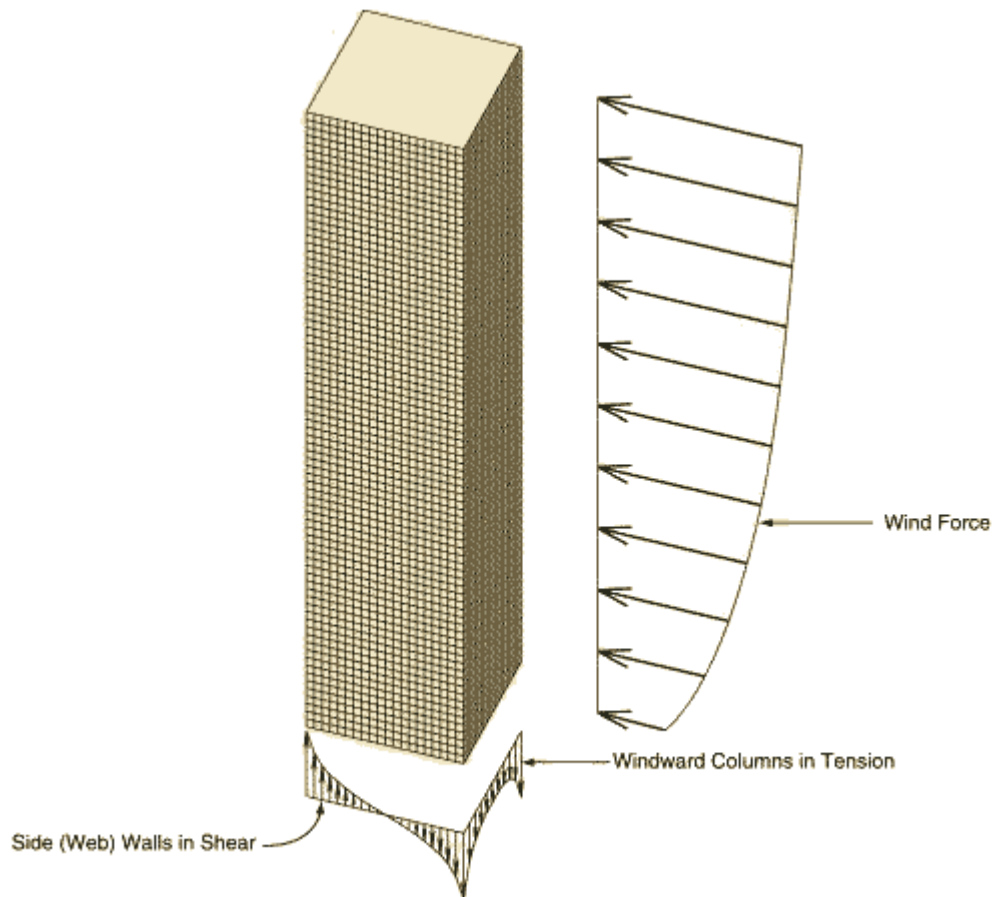
Figure 2-5 Structural tube frame behavior.
