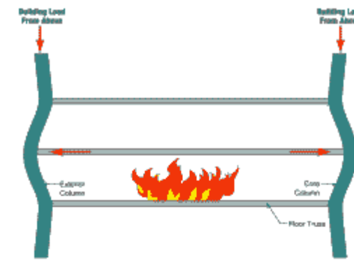
Figure 2-20 Expansion of floor slabs and building panels in heated conditions of columns and building exterior.
