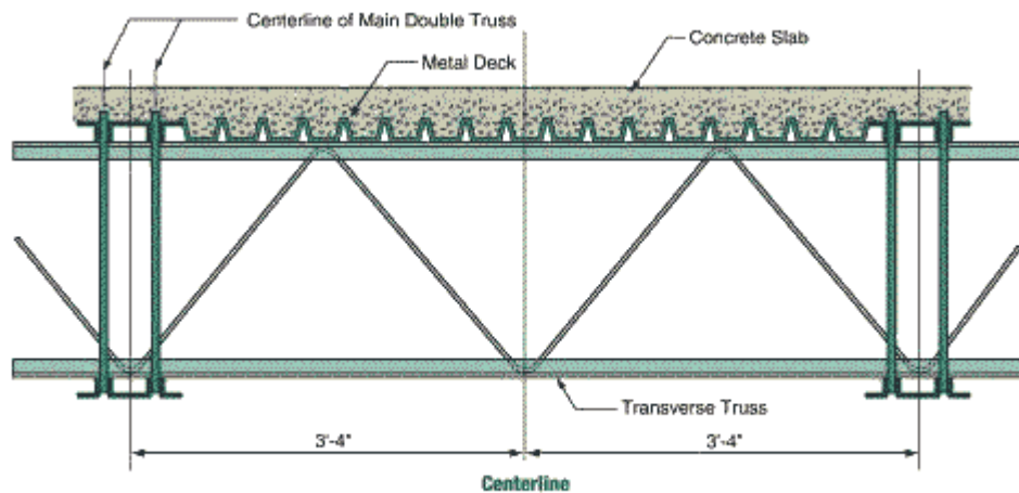
Figure 2-9 Cross-section through main double trusses, showing transverse truss.
