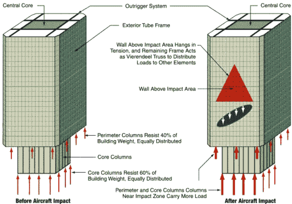
Figure 2-19 Redistribution of load after aircraft impact.
