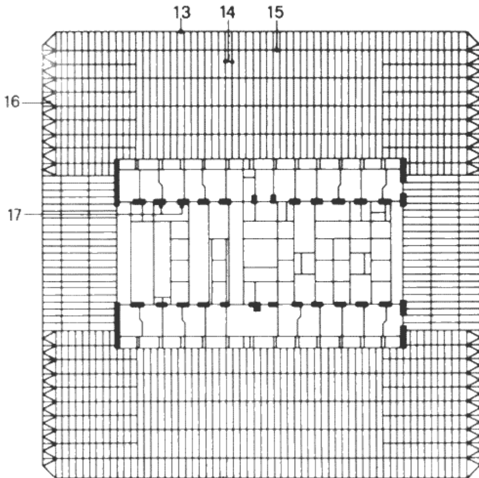
Figure 2-2-A Structural system for typical floor.
