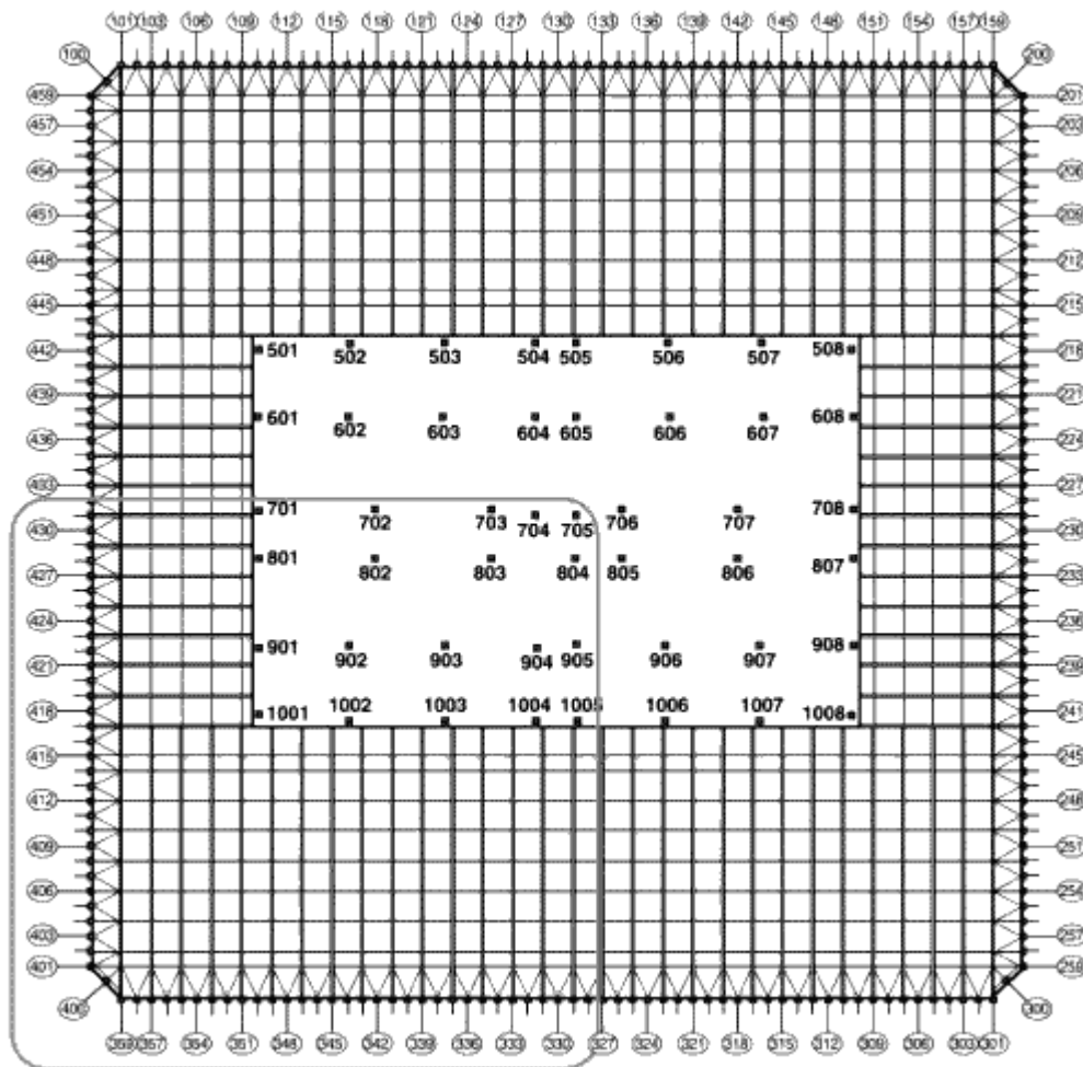
Figure 2-2 Representative structural framing plan, upper floors.
