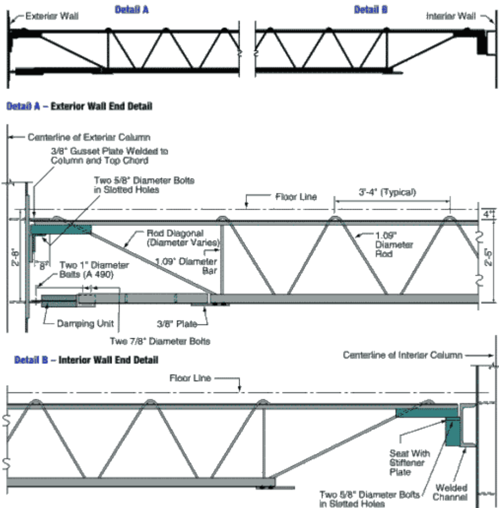
Figure 2-6 Floor truss member with detail of end connections.
