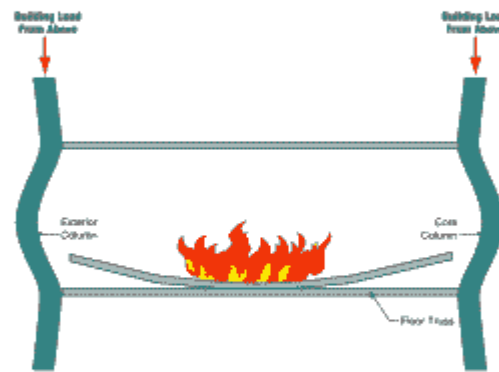
Figure 2-21 Buckling of columns under fire by loss of floor framing and compression.
