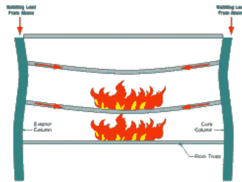
Figure 2-22 Catenary action of floor framing on several floors initiates column buckling failure.
