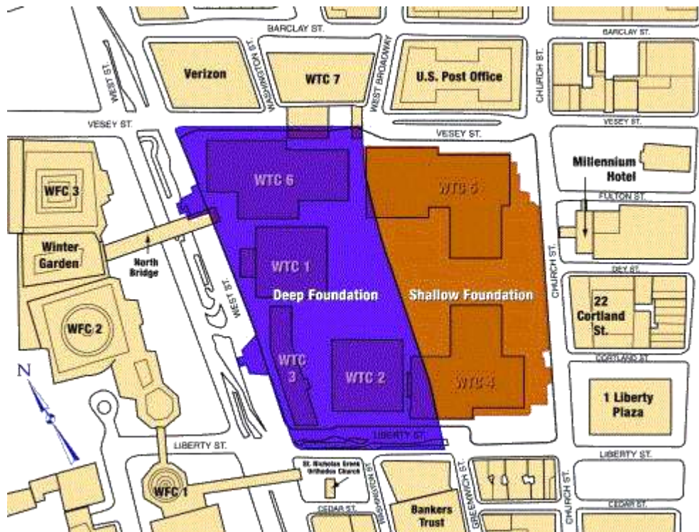
Figure 2-11. Location of subterranean structure.
